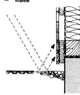
13 Replaceable construction of heavily weathered cladding
